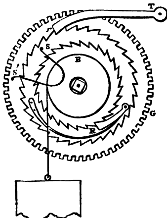
FIG. 14.—Harrison's Going-Ratchet.
