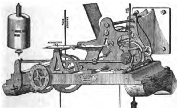
FIG. 19.—Clock at Meanwood Church, Leeds.
