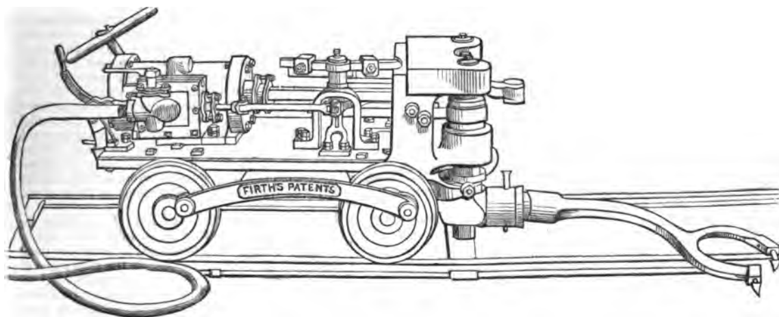
FIG. 13.—Firth's Coal-cutting Machine.
