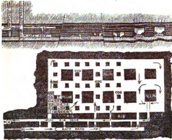
FIG. 11.—South Staffordshire method of working Thick Coal.
