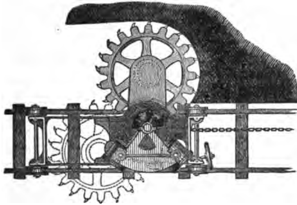
FIG. 14.—Winstanly & Barker's Coal-cutting Machine—Plan.
