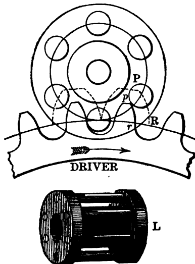
FIG. 24.—Lantern Pinion.
