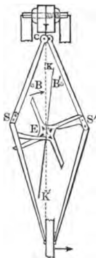
FIG. 12.—Four-Legged Gravity Escapement.
