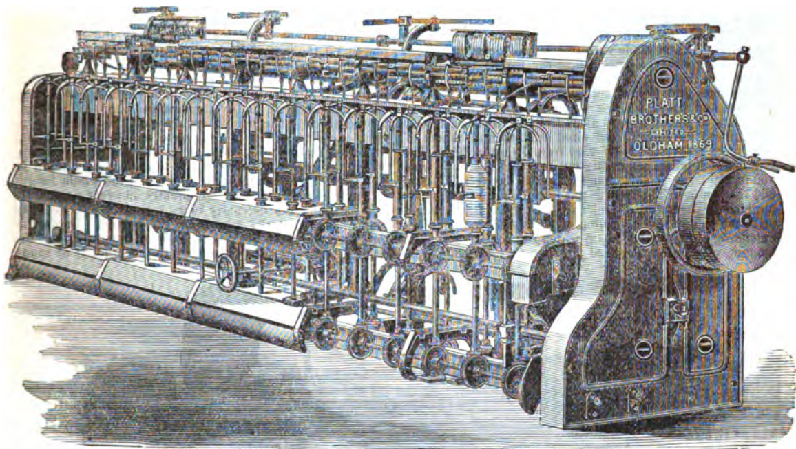
FIG. 9.—Slabbing Frame.
