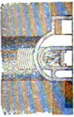
VENTILATING FURNACE SECTION
