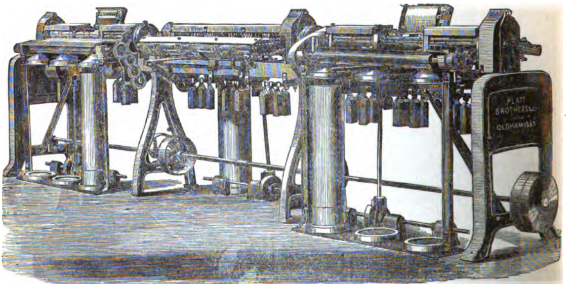
FIG. 8.—Drawing Frame.
