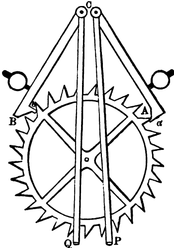
FIG. 10.—Mudge's Gravity Escapement.
