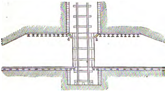
Fig. 5.—Pit eye, Cambois Colliery—Vertical Section.
