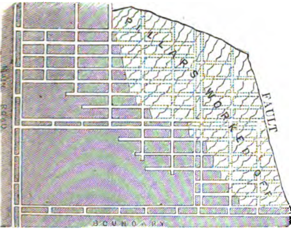
FIG. 9.—Lancashire method of working Coal.
