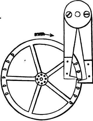
FIG. 6.—Pin-Wheel Escapement.
