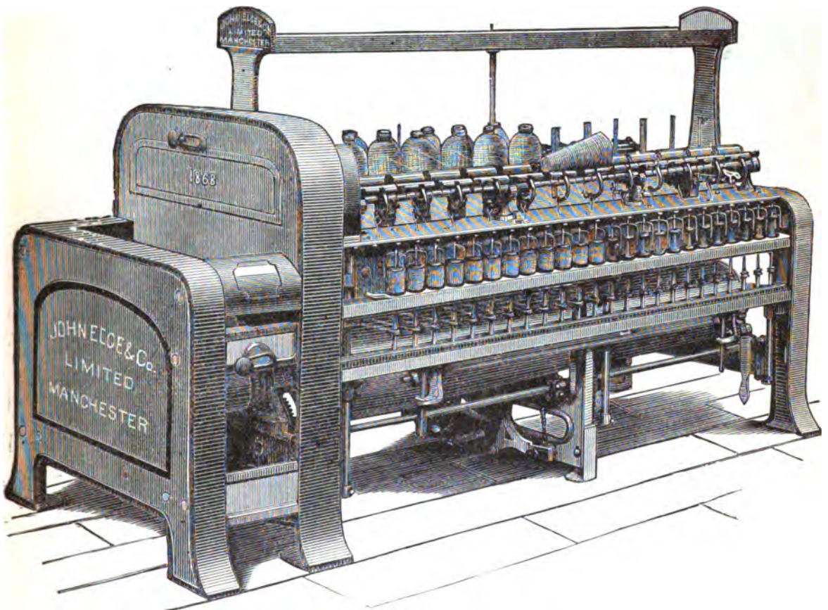
FIG. 12.—Throstle.
