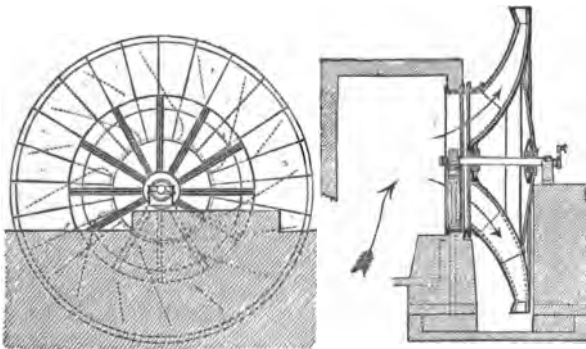
Fig. 18.—Waddle's Fan.
