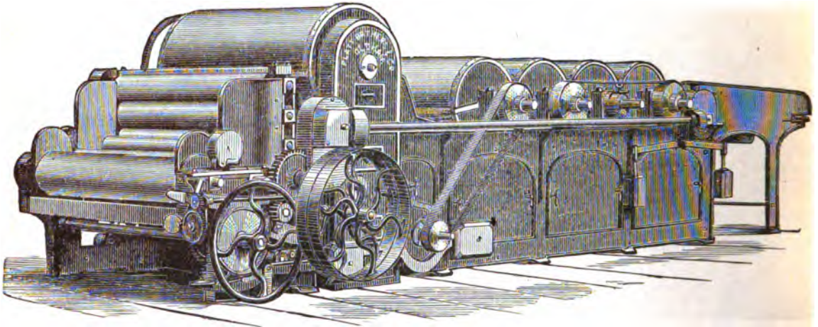
FIG. 3.—Three-cylinder Opener, Beater, and Lap Machine.
