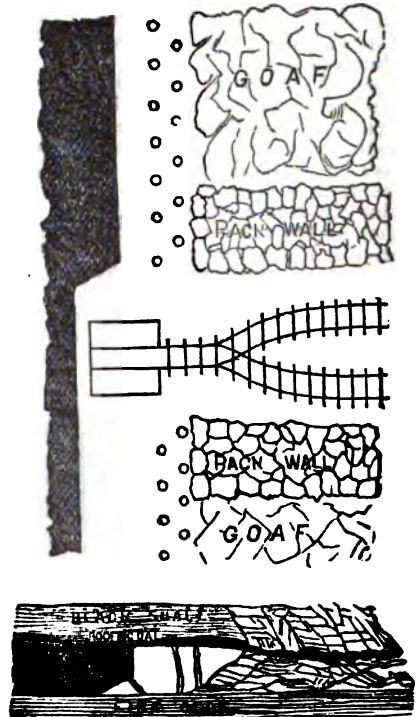
FIG. 12.—Long-wall working-face—Plan and Section.
