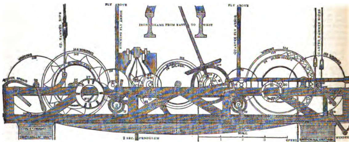
FIG. 27.—Section of Westminster Clock.
