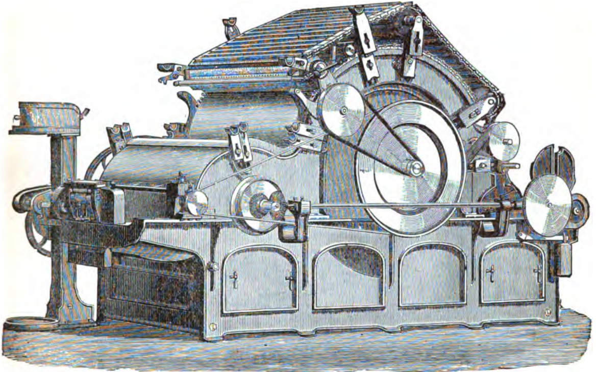
FIG. 5.—Self-stripping Flat Carding Machine.
