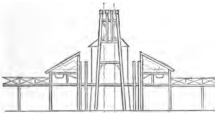
FIG. 24.—Transverse Elevation.
