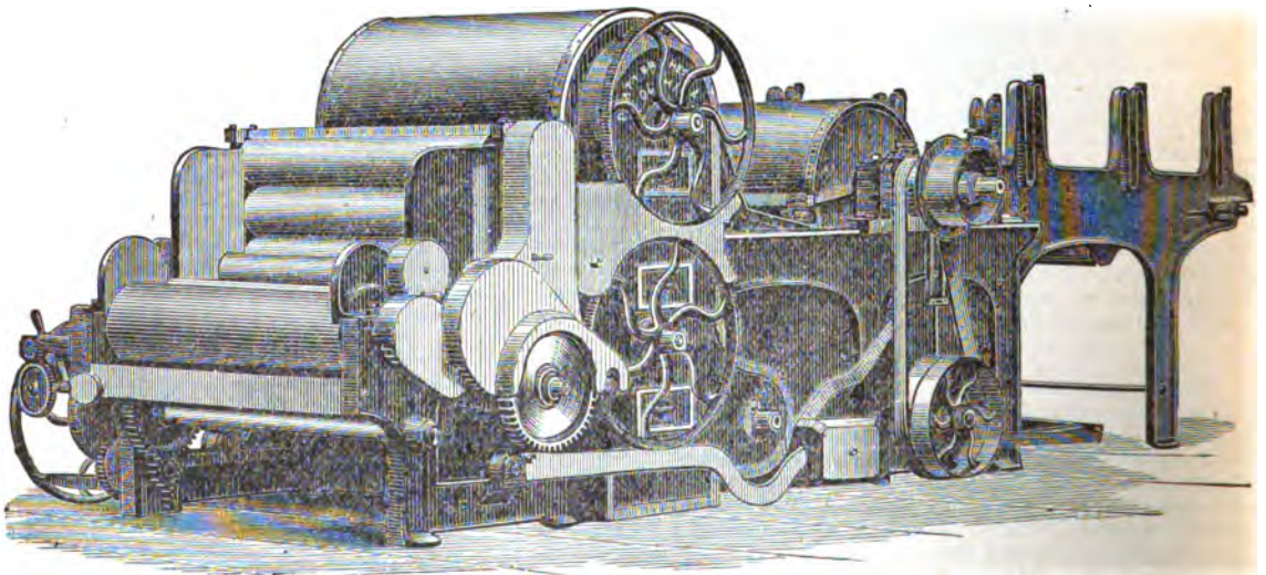
FIG. 4.—Single Scutcher and Lap Machine.
