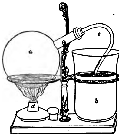
FIG. 3.—Napier's Coffee Apparatus.
