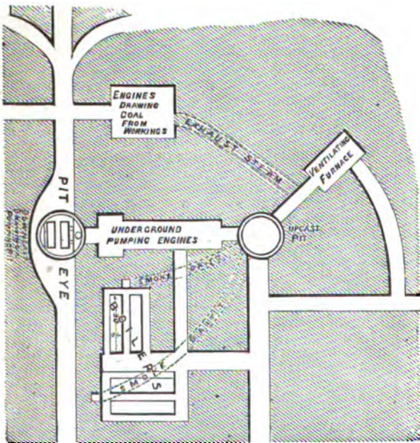
Fig. 6.—Pit bottom arrangements, Cambois Colliery.
