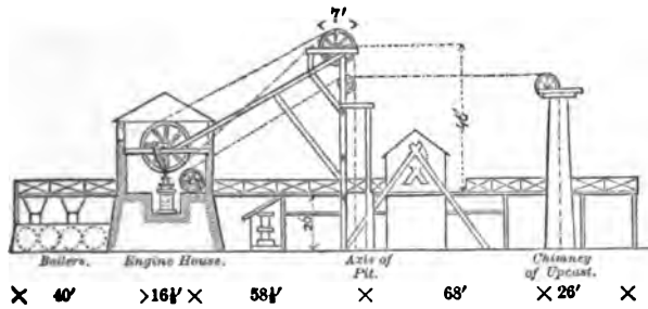
FIG. 22.—Elevation.
