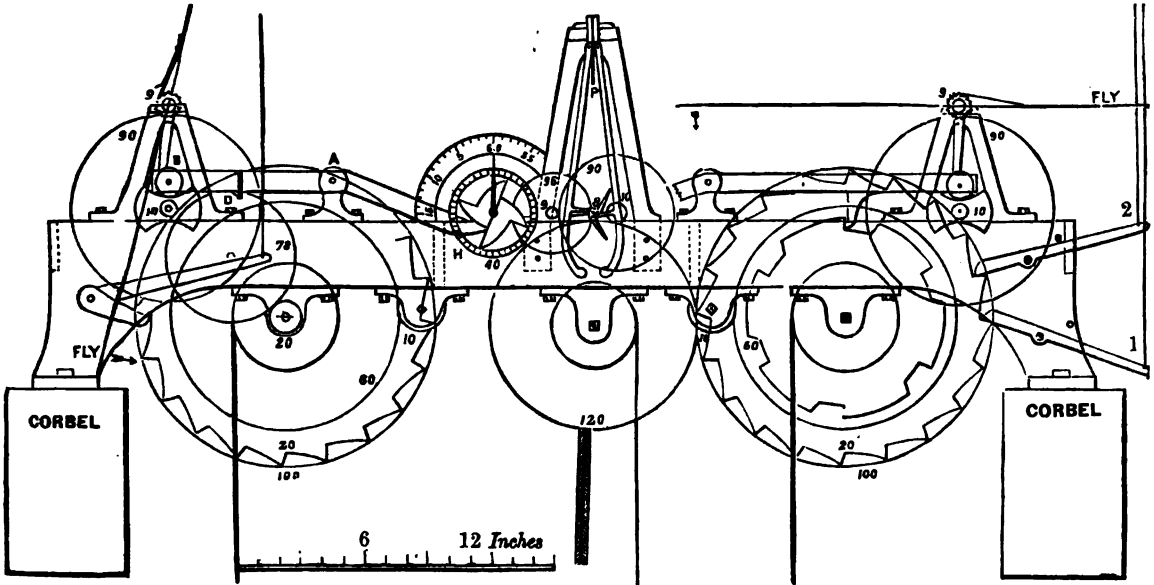
FIG. 22.—Front view of Turret Quarter Clock.
