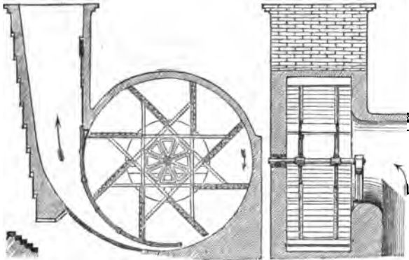
Fig. 17.—Guibal's Fan.
