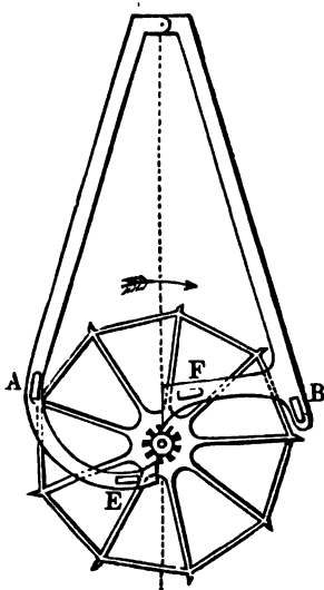
FIG. 11.—Bloxam's Gravity Escapement.
