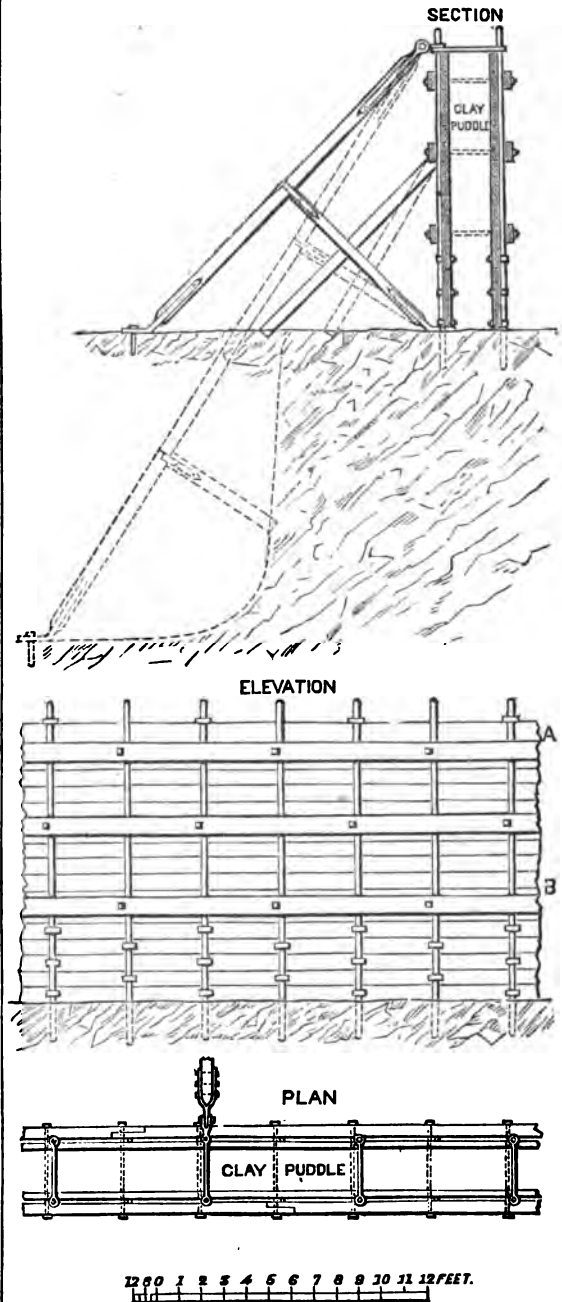
Fig. 3. Coffier-dam for Hard Bottom.
