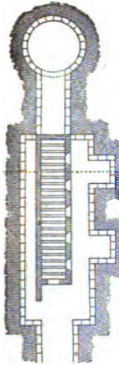
VENTILATING FURNACE PLAN
