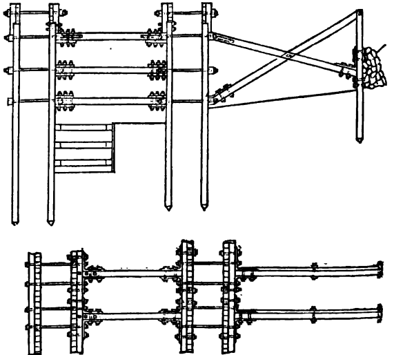
Fig. 2.—Coffer-dam used at Thames Embankment.
