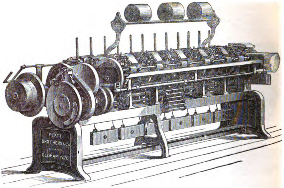
FIG. 7.—Combing Machine.
